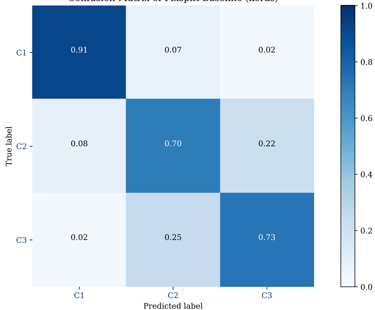
Confusion Matrix of Pixsplit Baseline (keras)
